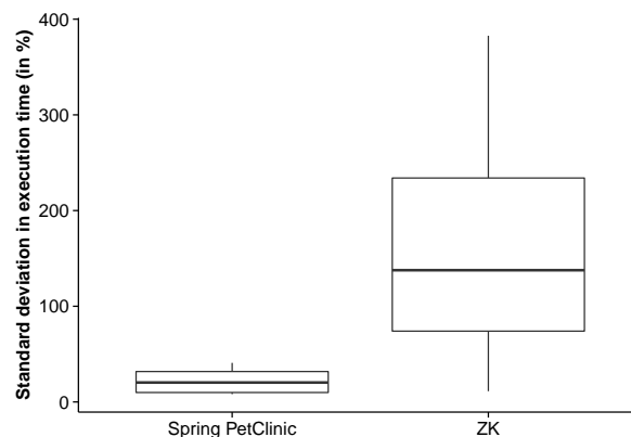
Figure 3: Standard deviation of relative difference in execution time (in %) for two randomly selected ORM configurations
